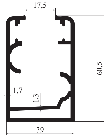
M 2107 - 1,153 kg/m
