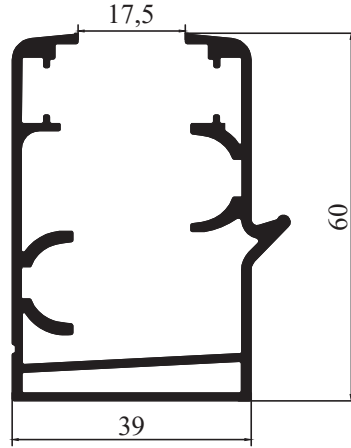
9134 - 1,157 kg/m
